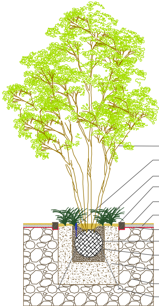
Fosse de Plantation 1/75
